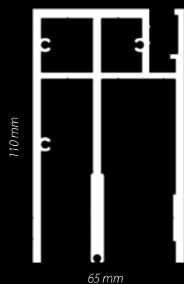
RUNNING PROFILE
