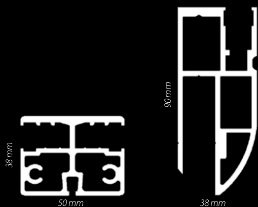
SUPPORT PROFILE
