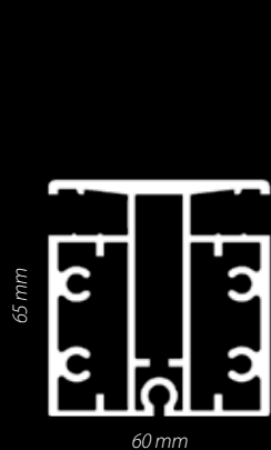
SUPPORT PROFILE
